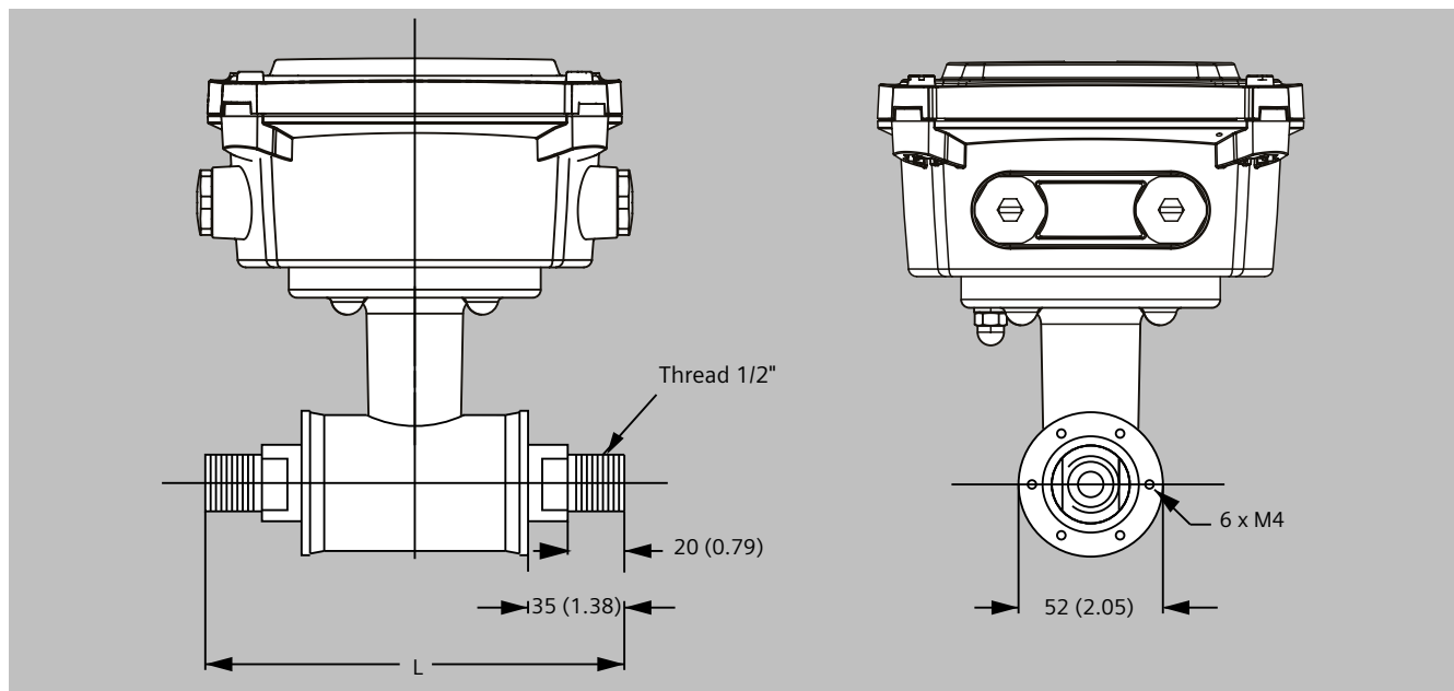
SITRANS FMS100 built-in length DN 2 ... 10 (1/12" ... 3/8") with adapters
